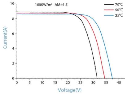
IV-CURVES of PV module SL260TU-30MD
