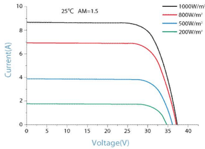
IV-CURVES of PV module SL260TU-30MD
