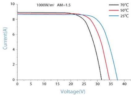
IV-CURVES of PV module SL245TU-30MDBK
