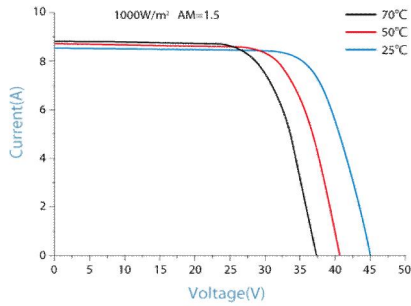
IV-CURVES of PV module SL295TU-36MDBK
