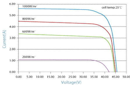
IV-CURVES of PV module SL205TU-36M
