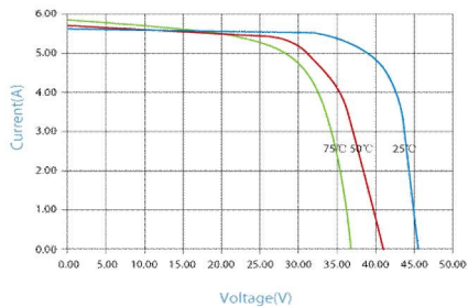
IV-CURVES of PV module SL190TU-36MBK
