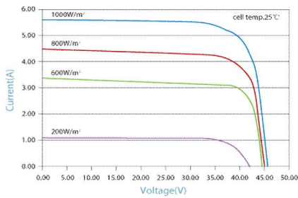
IV-CURVES of PV module SL200TU-36MBK
