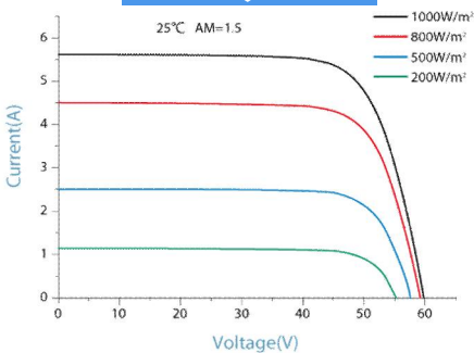
IV-CURVES of PV module SL250TU-48MBK
