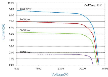
IV-CURVES of PV module SL230TU-30P
