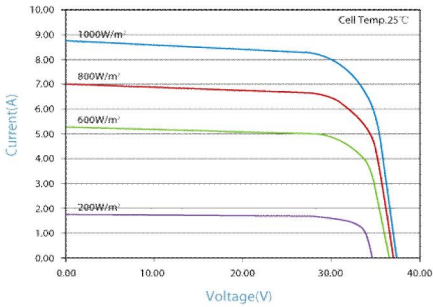
IV-CURVES of PV module SL235TU-30P
