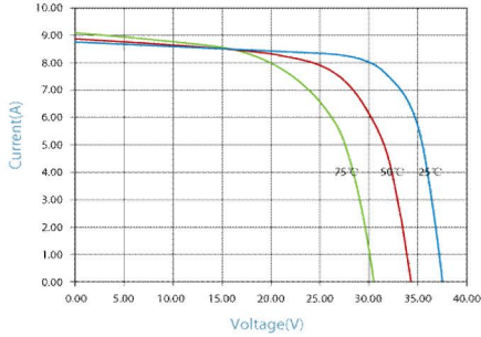
IV-CURVES of PV module SL240TU-30P
