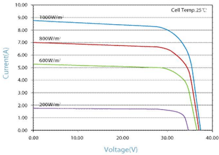
IV-CURVES of PV module SL245TU-30P
