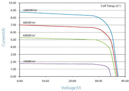
IV-CURVES of PV module SL250TU-30P
