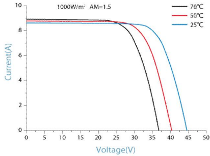
IV-CURVES of PV module SL285TU-36P
