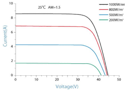
IV-CURVES of PV module SL295TU-36P
