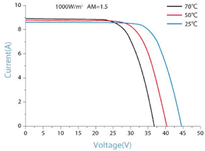
IV-CURVES of PV module SL295TU-36P
