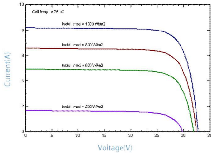
IV-CURVES of PV module SL210TU-27P
