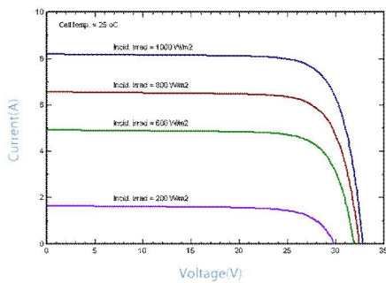
IV-CURVES of PV module SL215TU-27P
