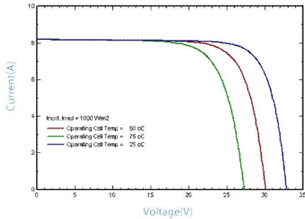
IV-CURVES of PV module SL225TU-27P
