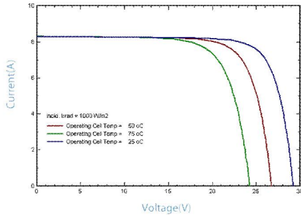
IV-CURVES of PV module SL190TU-24P
