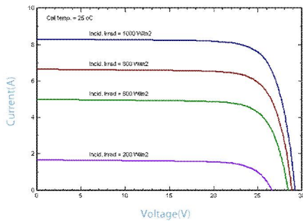
IV-CURVES of PV module SL200TU-24P
